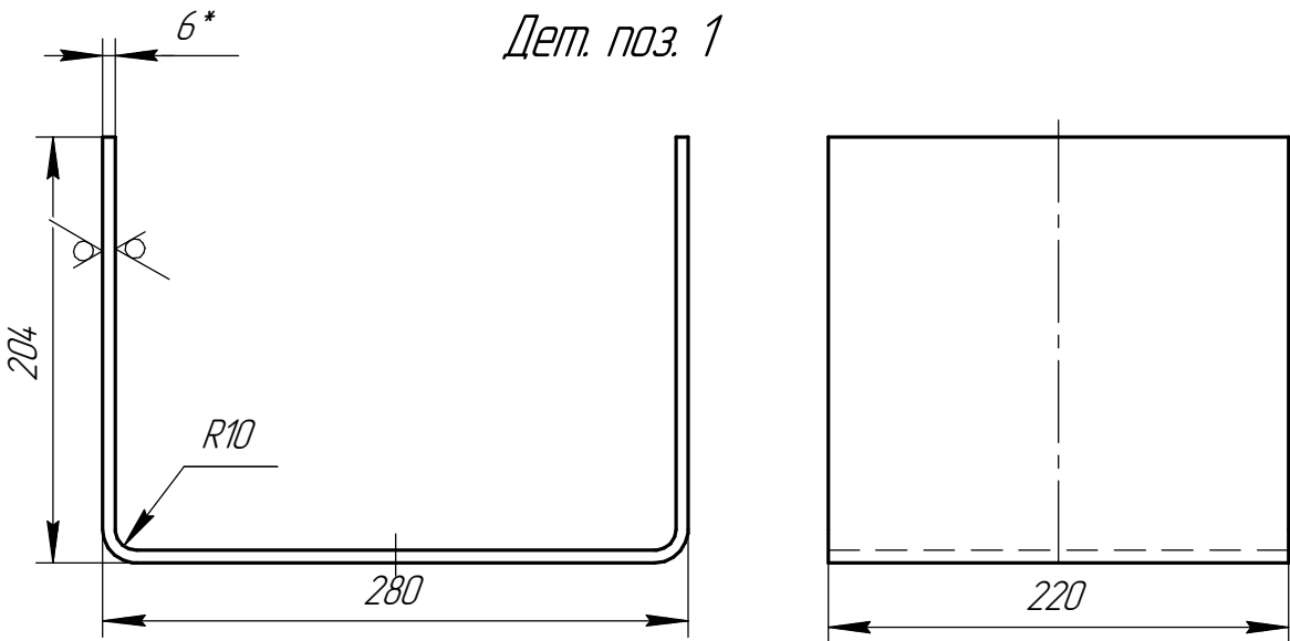
Q (1:5)
